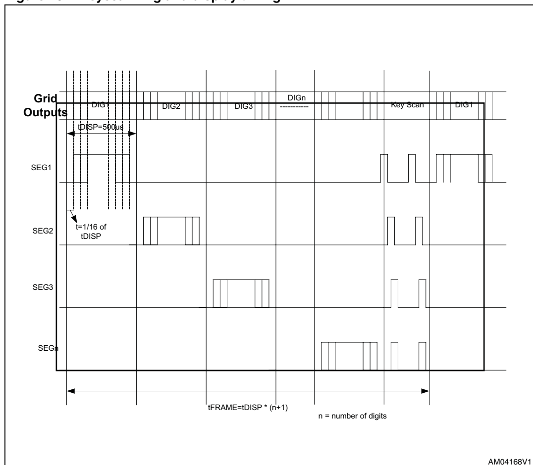
Figure 20. Keyscanning and display timing
